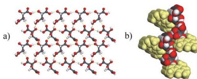
Fig. 3. Representations of a hydrogen-bonded sheet in the cocrystal of (caffeine)(D/L-tartaric acid): a) view perpendicular to the sheet, with caffeine molecules omitted for clarity; b) view parallel to the sheet, with caffeine molecules shown in space-filling fashion.
