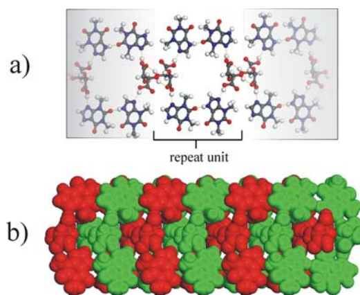
Fig. 2. a) A ball-and-stick model of a single hydrogen-bonded polymer ribbon with the repeat unit of the polymer shown; b) two interwoven ribbons in 2(theophylline)(DL-tartaric acid). For clarity each sheet is given a different colour.
