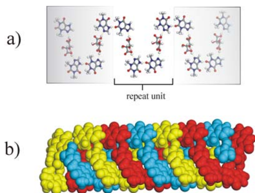
Fig. 1. a) A ball-and-stick model of a single hydrogen-bonded polymer ribbon with the repeat unit of the polymer shown; b) three interwoven ribbons in 2(theophylline)(D/L-tartaric acid). For clarity, each ribbon is given a different colour.
