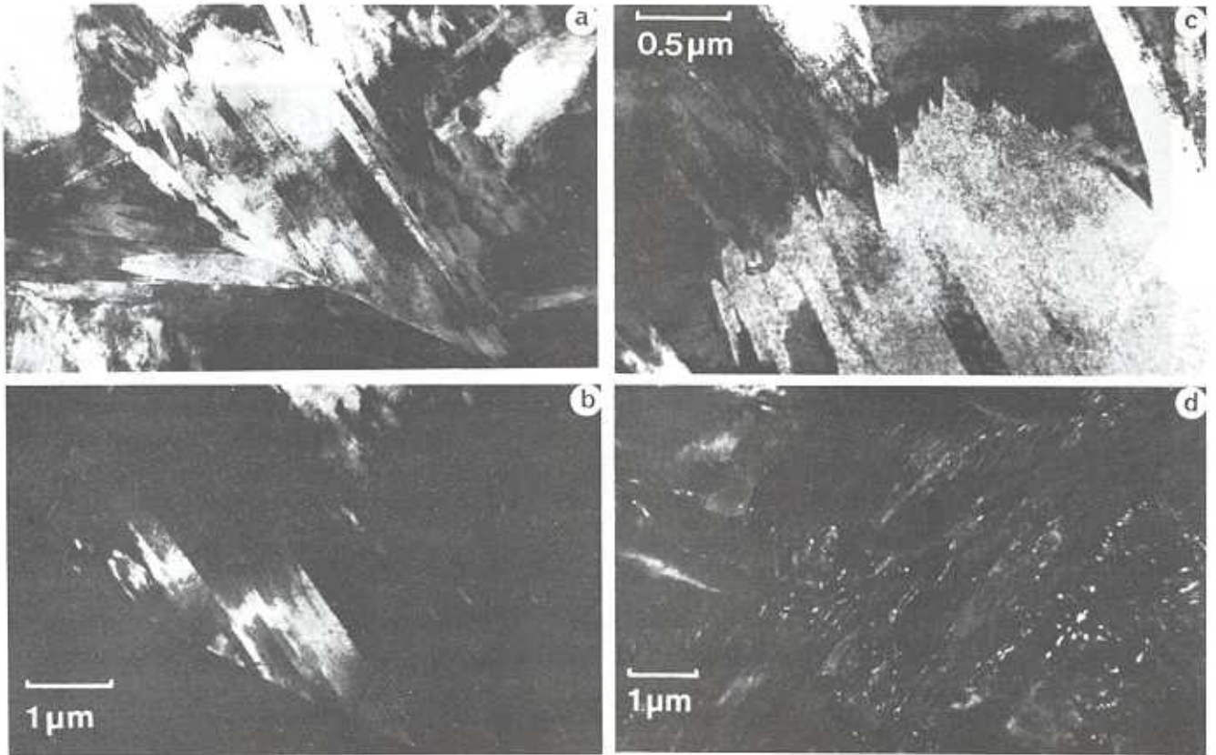
Figure 1 a) Lath Packet, Bright Field Image; b) Corresponding dark field image; c) Higher Magnification image of transformation front; d) Retained Austenite dark field image.
