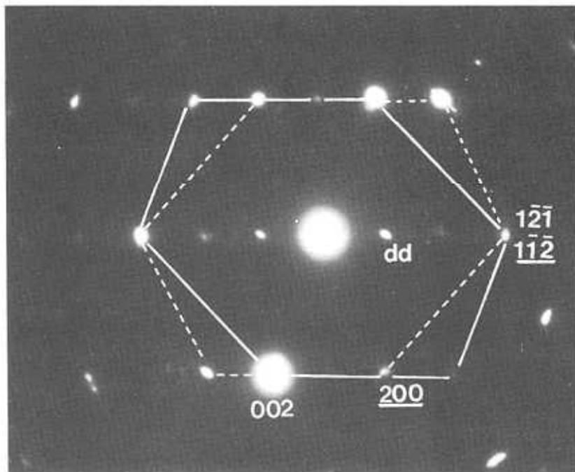
Figure 3 d) Corresponding diffraction pattern
