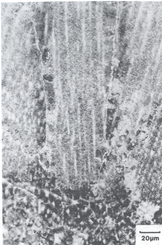
Fig. 3—Weld 1: Epitaxial growth at the fusion boundary. The austenite solidification structure may be seen within the columnar grains.
