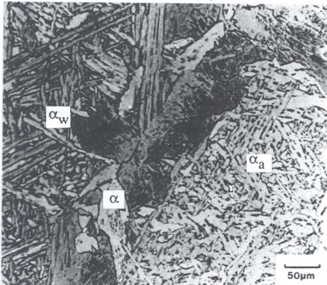
Fig. 6—Weld 2: Weld metal microstructure.
