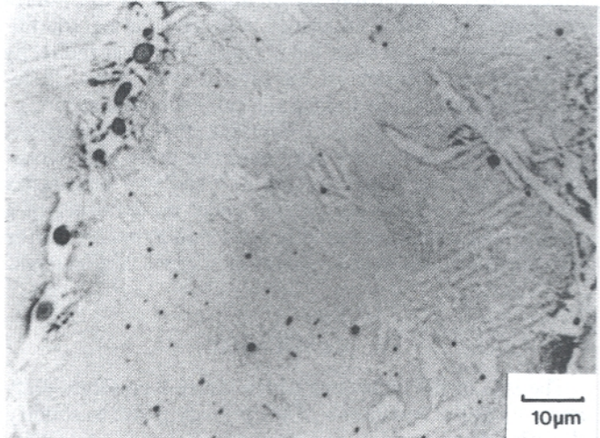
Fig. 4—Weld 1: Large inclusions are located predominantly at the grain boundaries of the solidifying phase (austenite).
