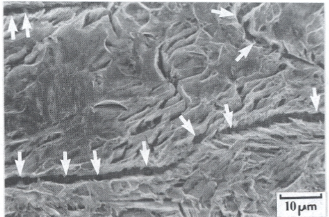
Fig. 5—Weld 1: Secondary electron image of deep-etched weld metal, showing inclusions (arrowed) at the columnar grain boundaries.
