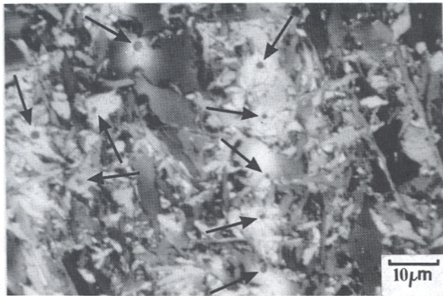
Fig. 7—Weld 2: Inclusions (arrowed) delineate the prior \delta grain boundaries.
