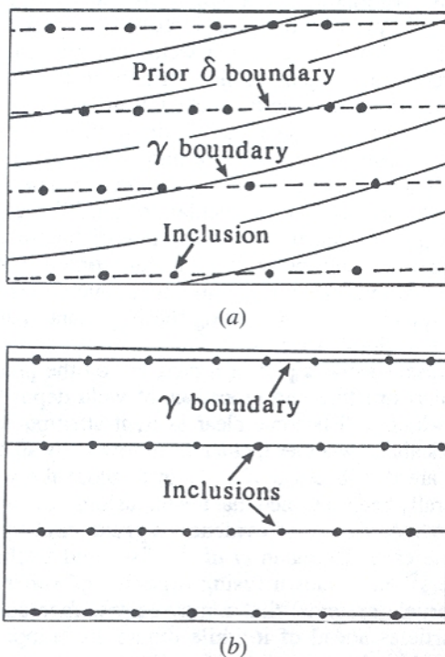
Fig. 1—Schematic diagram showing the location of inclusions in the microstructure of a weld for solidification as (a) \delta -ferrite and (b) austenite, assuming that the inclusions locate themselves preferentially at the cell boundaries during solidification. In (a) the prior \delta -ferrite boundaries and austenite boundaries diverge, since in arc welding the heat source is not stationary. 20
