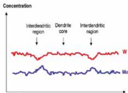
Fig. 18. Concentration profiles for W and Mo across dendrites in a Ni-based weld metal. Mo is enriched in interdendritic regions whereas W is depleted resulting in a more even distribution of alloying elements and thereby better corrosion resistance. Dendrite spacing is approximately 10 \mu\text{m} .
