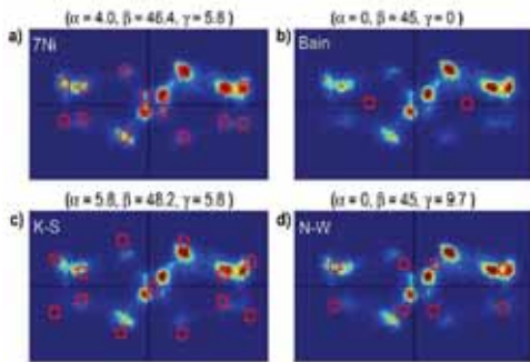
Fig. 12. Bain zone from a {111} experimental pole figure, colour-coded with respect to intensity. Theoretical poles for the different ORs 7Ni (best fit), Bain, Kurdjumov-Sachs (K-S) and Nishiyama-Wasserman (N-W) are marked with red circles in a)-d), respectively. The Euler angles are also given for each orientation.
