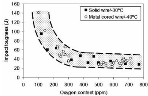
Fig. 2. Effect of oxygen content on Charpy-V impact toughness of supermartensitic weld metals. Weld metals produced with different welding processes and different consumables all fall within the same scatter band [6].
