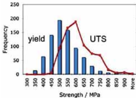
Fig. 1. Distribution of strength in ferritic steel weld metals, incorporating data from some 800 welding alloys. UTS stands for the ultimate tensile strength. Data from [4].
