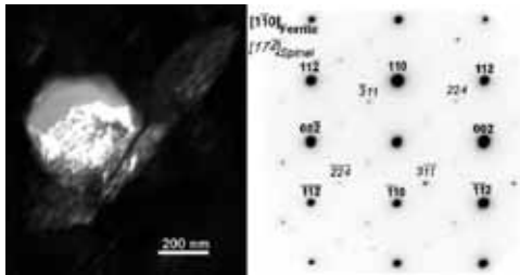
Fig. 9. a) Dark field transmission electron micrograph of an inclusion and an adjacent ferrite grain. b) The corresponding selected area electron diffraction pattern with indexed reflection for both the ferrite grain and the \text{MnTi}_2\text{O}_4 -spinel phase of the inclusion. Extra reflections are due to double diffraction.
