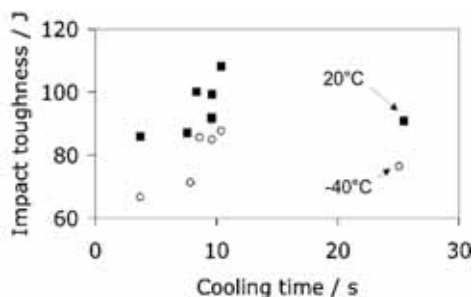
Fig. 7. Impact toughness as a function of cooling time ( \Delta t_{8/5} ) for a highly alloyed high strength weld metal.
