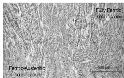
Fig. 14. Lean duplex weld metal with regions of Widmanstätten type austenite typical of a fully ferritic solidification (top) and regions having a morphology with ferrite located mainly interdentritically and forming an almost continuous network typical of mixed austenitic-ferritic solidification (bottom).
