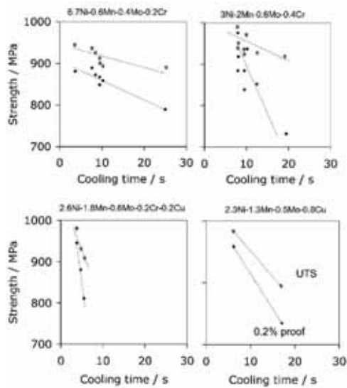
Fig. 4. Strength as a function of cooling time between 800 and 500°C for weld metals with Ni contents in the range 2.3–6.7 wt%, [18].
