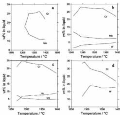
Fig. 17. ThermoCalc results from the Scheil calculations showing the concentration of elements in the liquid during solidification. At lower temperatures changes occur because of precipitation, which is probably too slow to take place in practise. The base composition was Ni - 0.05C, 0.5Si, 1Mn and 22Cr wt%, with varying amounts of Mo and W. a) 11Mo, b) 7.5Mo-5W, c) 5Mo-9W and d) 18W.
