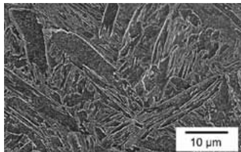
Fig. 3. Large coalesced bainite grains in the last bead of a 0.08C-10Cr-1Ni-0.3Mo wt% high strength weld metal with 910 MPa in yield strength.
