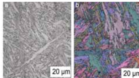
Fig. 11. (a) LOM micrograph showing the etched microstructure of a 7Ni weld metal. (b) EBSD orientation map from the same microstructure.
