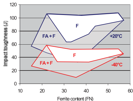
Fig. 15. Impact toughness scatter bands for lean duplex weld metals with a fully ferritic solidification (F) and those with regions having a morphology with ferrite located mainly interdendritically and forming an almost continuous network typical of mixed austenitic-ferritic solidification (FA). The minimum values and scatter increase significantly with mixed mode solidification.
