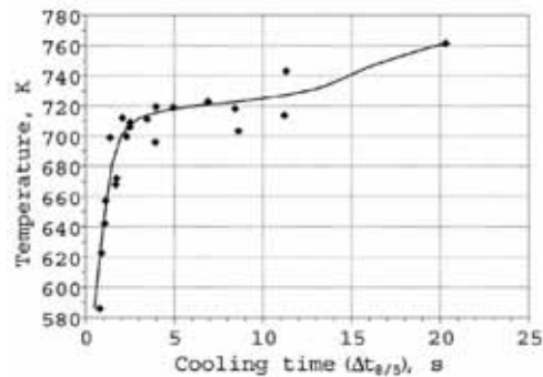
Fig. 6. Experimental CCT-diagram for OK 75.78 displaying transformation start temperatures as a function of cooling time between 800°C and 500°C. Transformation temperatures gradually increase with cooling time above 3 s and decrease rapidly for shorter cooling times.
