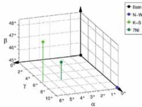
Fig. 13. Euler space representation of the orientation relation between austenite and ferrite in a 7Ni weld metal. Common rational relationships are displayed for reference.
