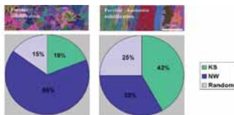
Fig. 16: EBSD orientation maps (top) and classification of austenite/ferrite boundary orientations (below) for weld metals with a fully ferritic solidification (left) and mixed ferritic-austenitic solidification (right). More phase boundaries had a random orientation relationship after mixed mode solidification. The NW relationship was most frequent after fully ferritic solidification whereas KS was more common after a mixed mode solidification.
