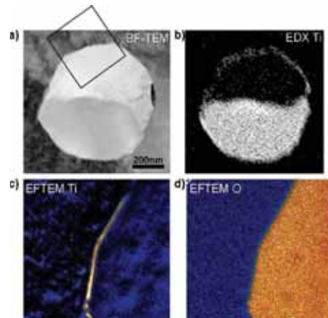
Fig. 10. Bright field transmission electron micrograph of an inclusion. An EDX titanium map of the inclusion is shown in b). Energy filtered transmission electron micrographs of titanium and oxygen elemental maps are shown in c) and d), respectively. The maps were recorded over the area marked with a black square in a).
