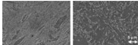
Fig. 5. FEGSEM micrographs presenting an overview of the as-deposited last bead microstructure for two different cooling times. Lower bainite, martensite and coalesced bainite are the main constituents in the rapidly cooled weld metal on the left, whereas the more slowly cooled structure consists largely of upper bainite.
