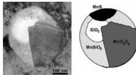
Fig. 8. a) Bright field transmission electron micrograph of an inclusion. b) Schematic representation of the inclusion, showing the morphology of present phases.
