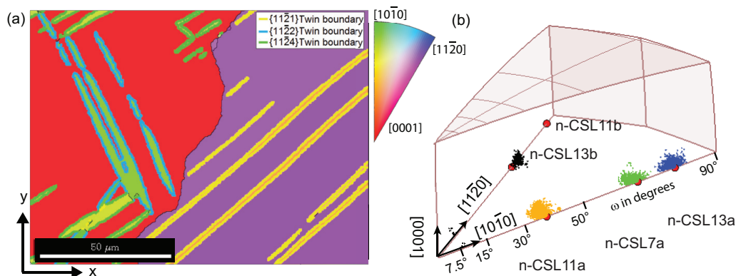
Figure 10: (a) Twinned microstructure of ballistically tested pure Ti, adapted from [78]. The loading axis is parallel to the x-direction. IPF colours are with respect to the x-axis. (b) Fundamental zone ( f/24 , cf. Table 1) for 6/mmm misorientations. Clusters of grain boundary misorientations corresponding to \{11\bar{2}1\} , \{11\bar{2}2\} and \{11\bar{2}4\} twin boundaries are coloured and highlighted in the microstructure. The grain boundary misorientation is close to the \{10\bar{1}1\} twinning OR and is coloured black.
