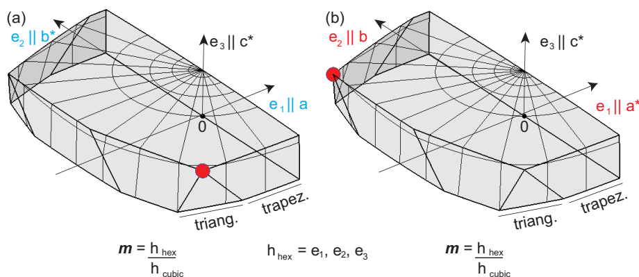
Figure 15: Influence of hexagonal reference frame on fundamental zone for cubic-hexagonal misorientations (a) first setting, cub: standard, hex: standard. Blackburn relation at lower corner (b) The second setting, cub: standard, hex: \mathbf{e}_2 = \mathbf{b}/b, \mathbf{e}_3 = \mathbf{c}^*/c^* leads to a rotation of the Blackburn relation to the upper corner, however, the domain is unchanged.
