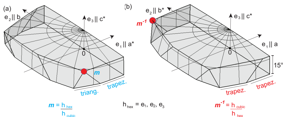
Figure 16: Influence of the sequence on the fundamental zone: Either (a) cubic-hexagonal misorientations ( e_1 - e_3 refer to cubic reference frame) or (b) hexagonal-cubic misorientations ( e_1 - e_3 refer to hexagonal reference frame) are formed. Note the change in geometry in (b) compared to (a) and the changed location of the Blackburn relation. Both FZ were formed with the standard definition for hexagonal symmetry as was done previously in Figure 15a.
