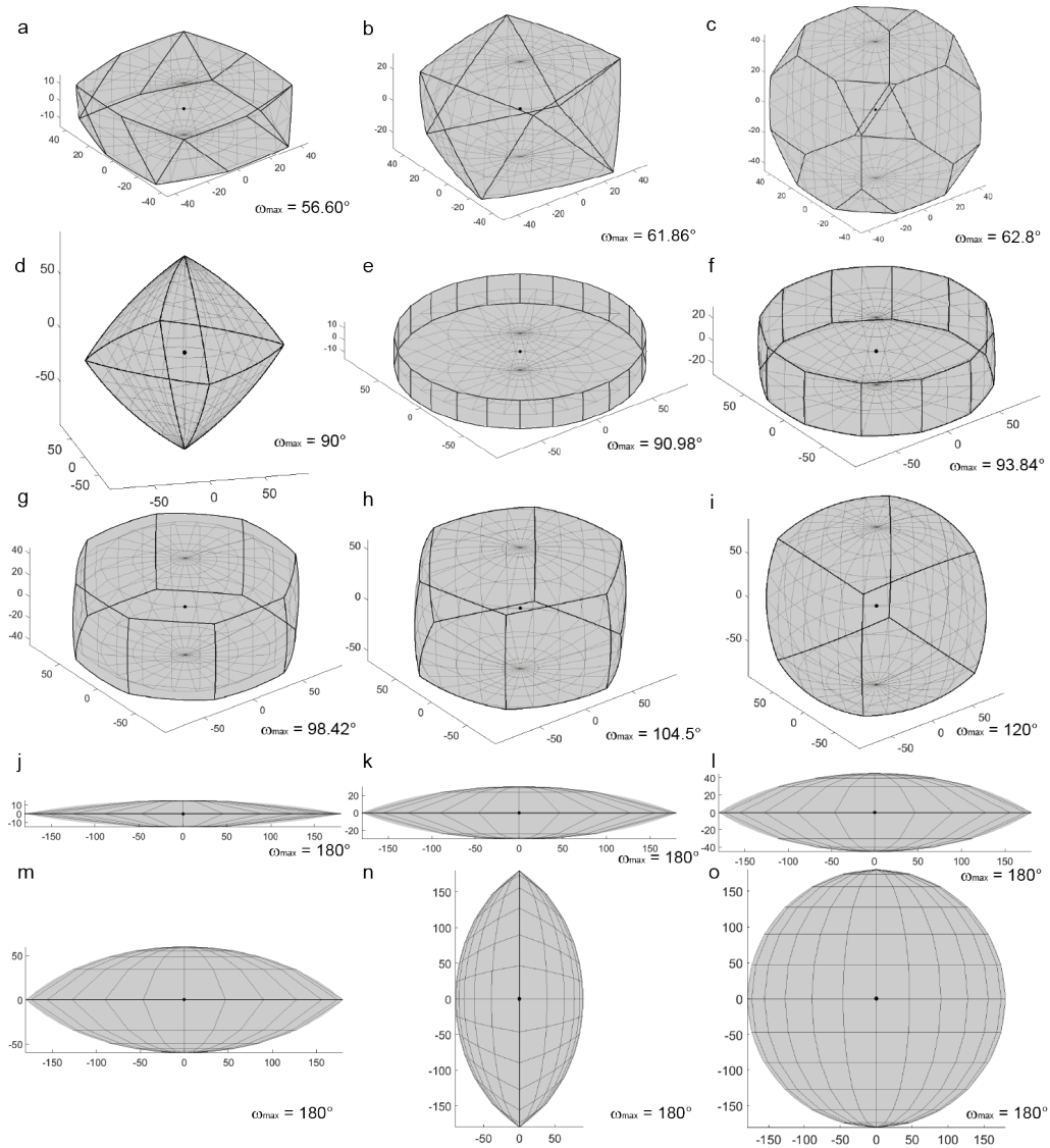
Figure 5: Domain geometries in axis-angle representation with the reference misorientation at the origin (marked with a point). Combinations of point group symmetries leading to fundamental zones that are one of these domain geometries or a section of it are provided in Table 1.
