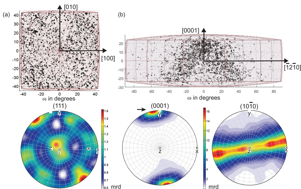
Figure 11: Fundamental zones for orientations of (a) \gamma phase (domain c) and (b) \eta phase (domain f). Pole figures are shown for comparison below the corresponding fundamental zone, plotted as orientation density function. Both representations can be used to identify the strong texture displayed by the \eta phase.
