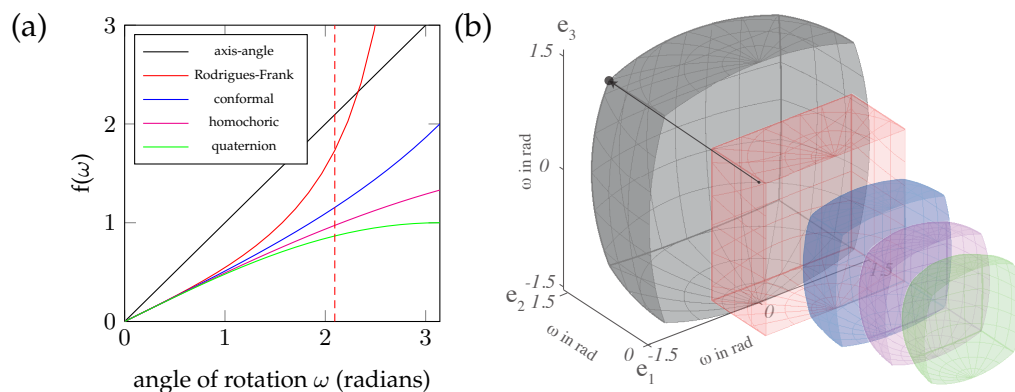
Figure 2: (a) The scaling function for five neo-Eulerian orientation mappings as a function of the rotational angle. The maximum angle for 222 symmetry is 2\pi/3 radians ( 120^\circ ) in [111] direction (indicated by red dotted lines). (b) Sectioned fundamental zone for 222 symmetry in each of the five neo-Eulerian mappings, illustrating differences in geometry.
