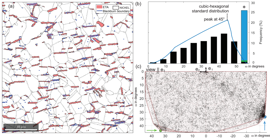
Figure 12: (a) Phase map with grain boundaries in black and interphase boundaries with Blackburn OR in blue, (b) misorientation angle distribution (1D) indicating high density at angles > 50^\circ ; *max. angle is 56.60^\circ . For comparison: random distribution in blue. (c) 3D misorientation distribution of \gamma - \eta phase boundary in the appropriate fundamental zone (a/4), indicating that both, Blackburn and Crawley OR contribute to the high frequency at the max. angle.
