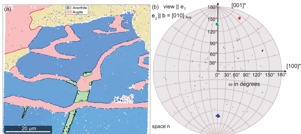
Figure 14: (a) Orientation map showing the occurrence of three orientations for anorthite (yellow, green and blue) and one for augite (pink) with the respective phase boundaries coloured red, green and blue. (b) Augite-anorthite misorientations in the appropriate fundamental zone (domain n); misorientation clusters coloured in accordance with phase boundaries in (a).
