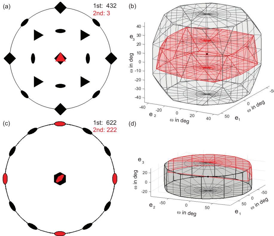
Figure 4: Stereographic projections (a,c) of symmetry elements and corresponding symmetry reduced fundamental zones of axis-angle space (b,d) for: (a,b) misorientations of crystals with point group (PG) 432 and combination of PGs 432 - 3 (c,d) misorientations of crystals with PG 622 and combination of 622 - 222.
