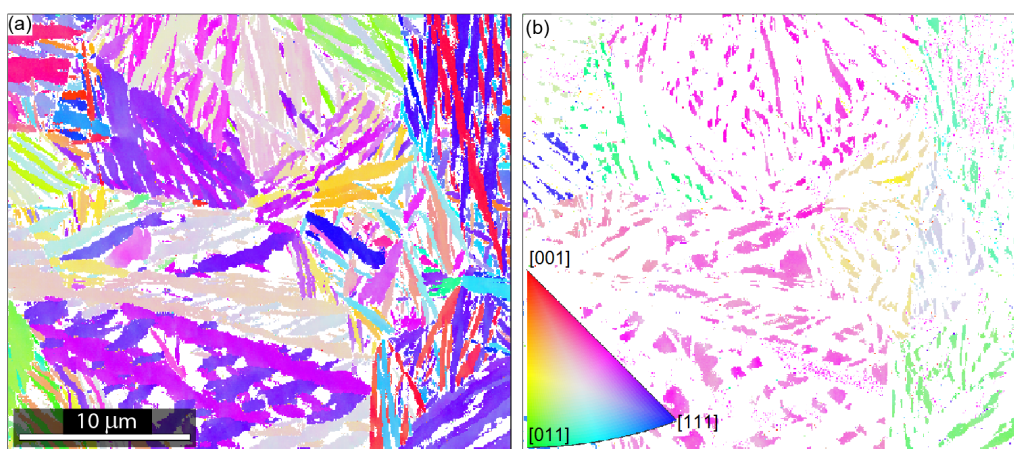
Figure 8: Nanostructured bainite [69], IPF colour code with regard to z-axis for both maps in the inlay (a) Orientation map of ferrite laths in IPF colours. Several orientations of laths occur within a prior austenite grain. (b) Orientation map of the retained austenite phase in IPF colours.
