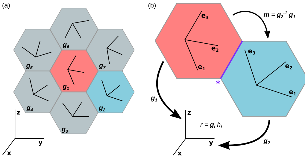
Figure 1: (a) Orientations g_i of crystallographic axes in each structural element (pixel, voxel, or grain) with respect to an external reference frame. (b) Orientations g_i as transformations from the crystal reference frames h_i into the specimen reference frame r and misorientation m describing transformation between crystal reference frames across a boundary element (starred).
