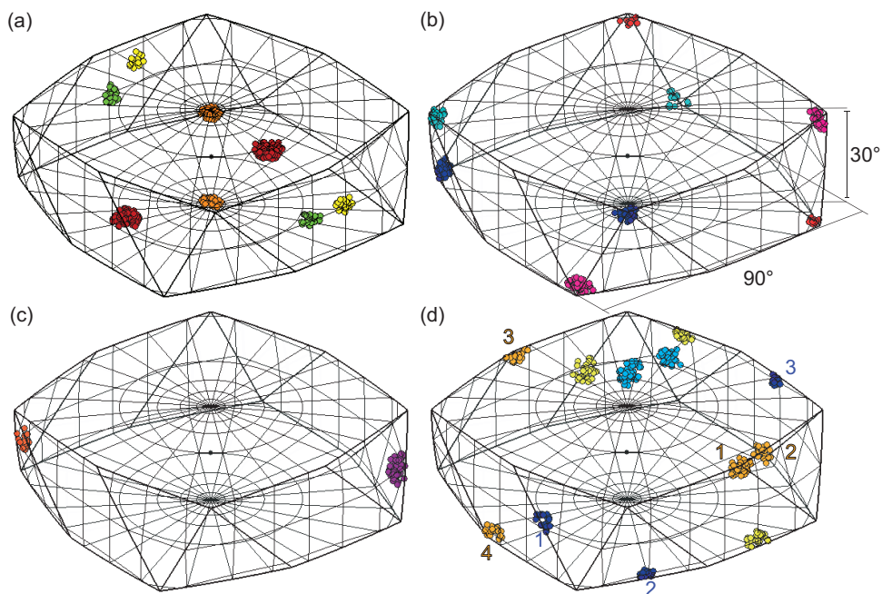
Figure 6: Properties of misorientation clusters situated at the bounding surface of the cubic ( m\bar{3}m ) to trigonal ( \bar{3} ) fundamental zone (domain a). This is illustrated by colouring similar misorientations with equal colours for each image separately. (a) Clusters reappearing at an opposite boundary face, either directly opposite or opposite and rotated; (b) Clusters at a corner reappearing at another corner; (c) Clusters that do not reappear in a different position; (d) Clusters at edges and triple points can split into more than two clusters.
