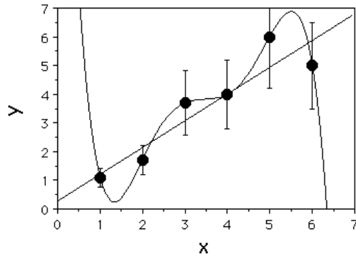
Fig. 4: A complicated model may overfit the data. In this case, a linear relationship is all that is justified by the noise in the data.
