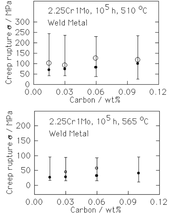
Fig. 7: Calculated (filled circles with error bars) and measured (open circles) stress rupture data for 2.25Cr1Mo weld metal.
