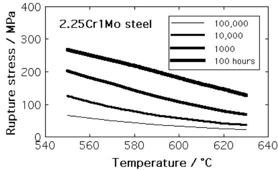
Fig. 8: Calculated stress rupture data for 2.25Cr1Mo weld metal.
