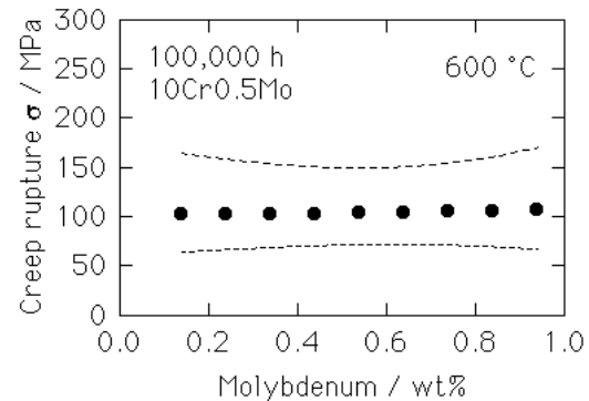
Fig. 5: Creep rupture stress at 600 °C and 100,000 h for 10Cr-0.5Mo type steel
