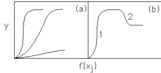
Fig. 3: (a) Three different hyperbolic tangent functions; the “strength” of each depends on the weights. (b) A combination of two hyperbolic tangents to produce a more complex model.
