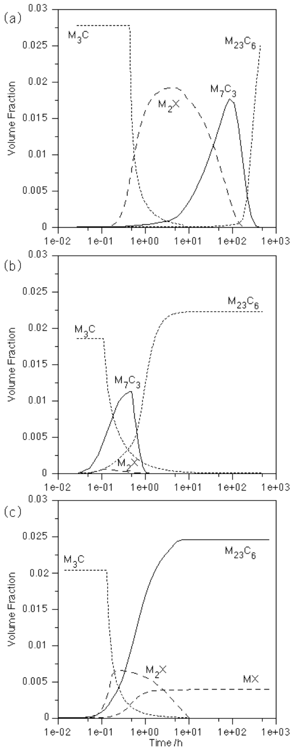
Fig. 2: The predicted evolution of precipitate volume fractions at 600 °C for three power plant materials (a) 2\frac{1}{4} Cr1Mo (b) 3Cr1.5Mo and (c) 10CrMoV.
