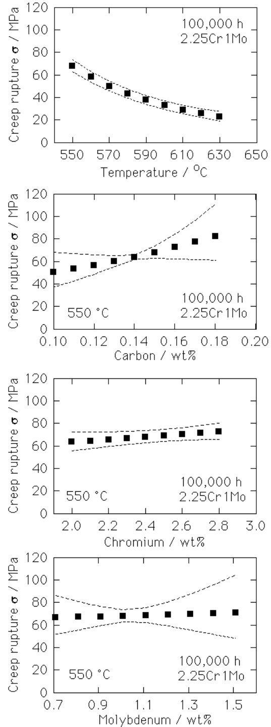
Fig. 6: Creep rupture stress at 600°C and 100,000 h for 2.25Cr-1Mo type steel
